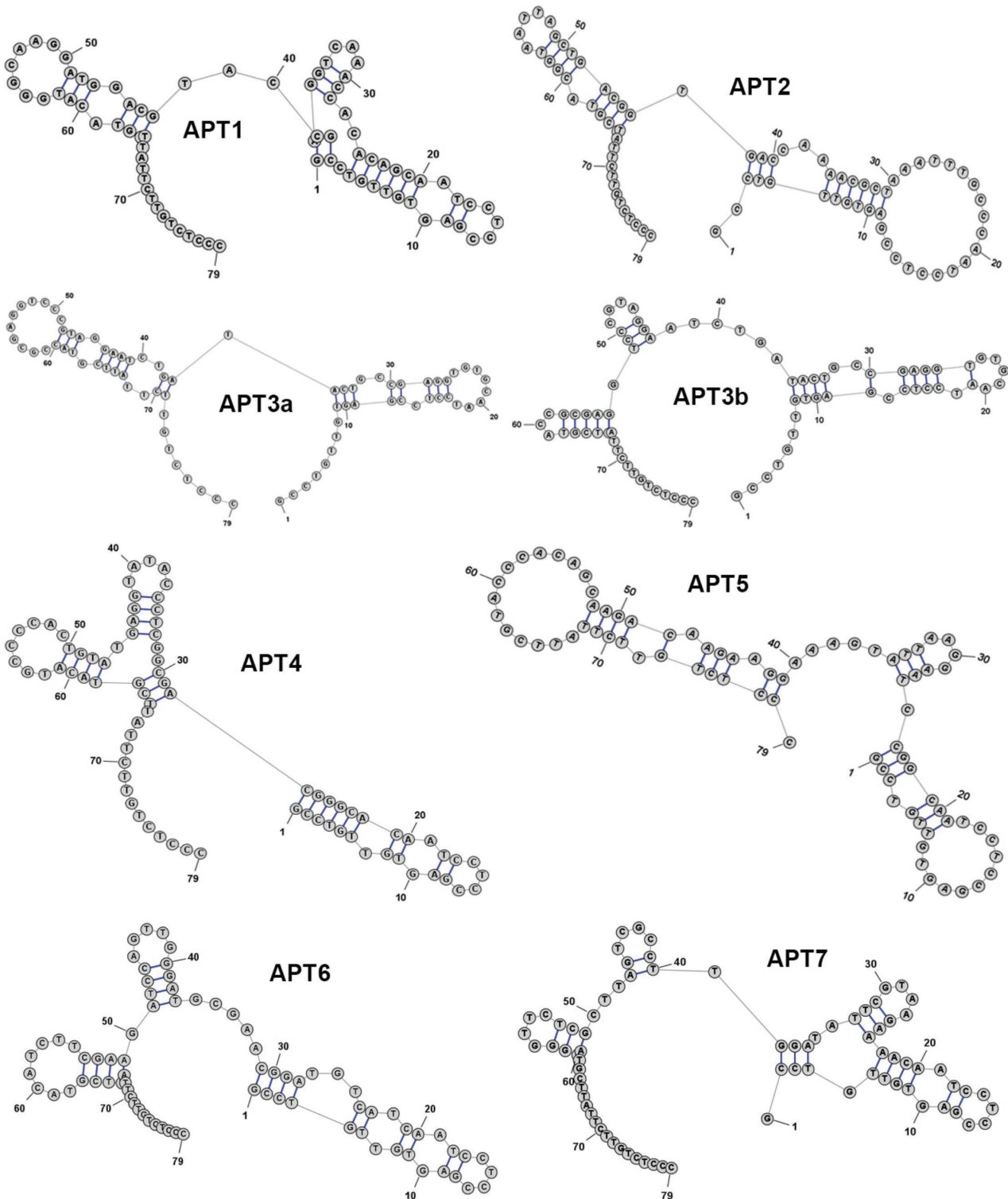
Figure 5. Configurations of the representative aptamers (graphed by RNAstructure 6.2 software). Ionic strength was set to the physiological conditions (144 mM Na + ) and temperature was set to 21 °C.
